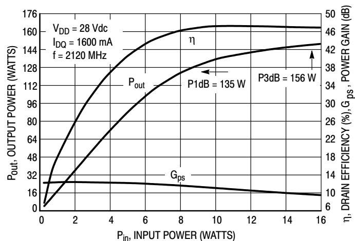
Figure 5. CW Performance
