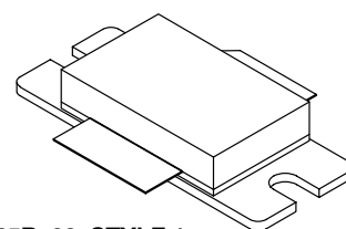
CASE 465B-03, STYLE 1 NI-880 MRF21125R3
