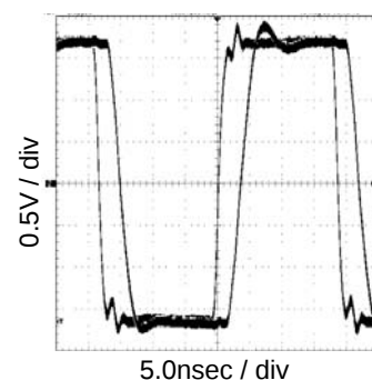
Fig.26 Buffer delay(IN→OUT2) VDD=3.3V,CL=50pF
