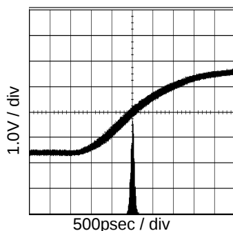
Fig.4 33.868MHz Period-Jitter VDD=3.3V,CL=32pF
