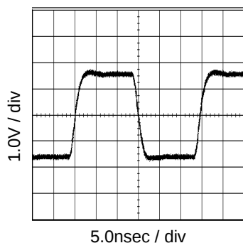
Fig.3 33.868MHz output waveform VDD=3.3V,CL=32pF
