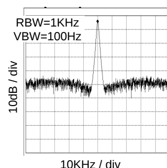
Fig.5 33.868MHz spectrum VDD=3.3V,CL=32pF
