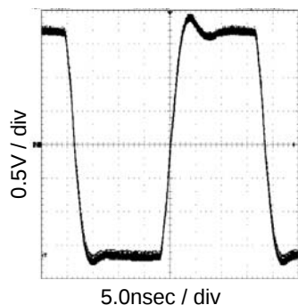
Fig.24 Buffer skew output waveform VDD=3.3V,CL=50pF
