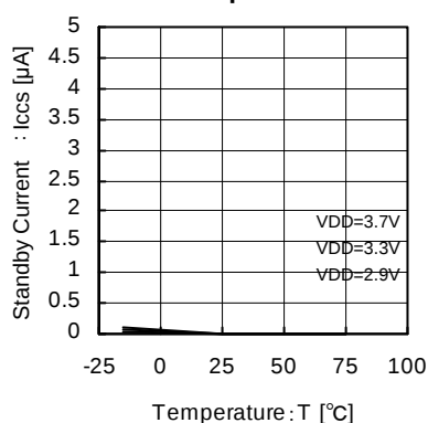
Fig.66 Power-down Standby Current
