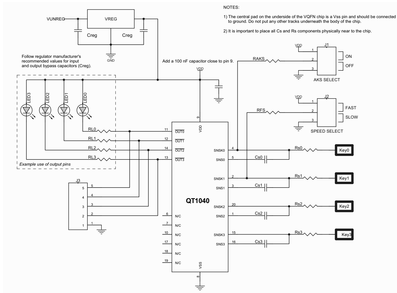
Figure 1-1. Typical Circuit
