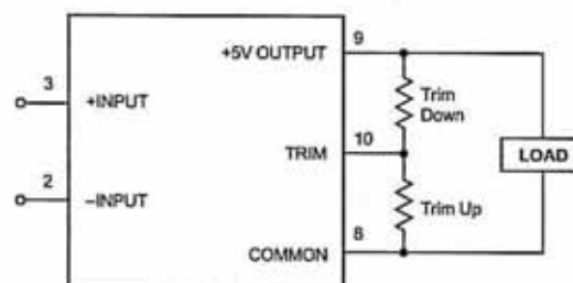
Figure 8. Trim Connections Using Fixed Resistors
