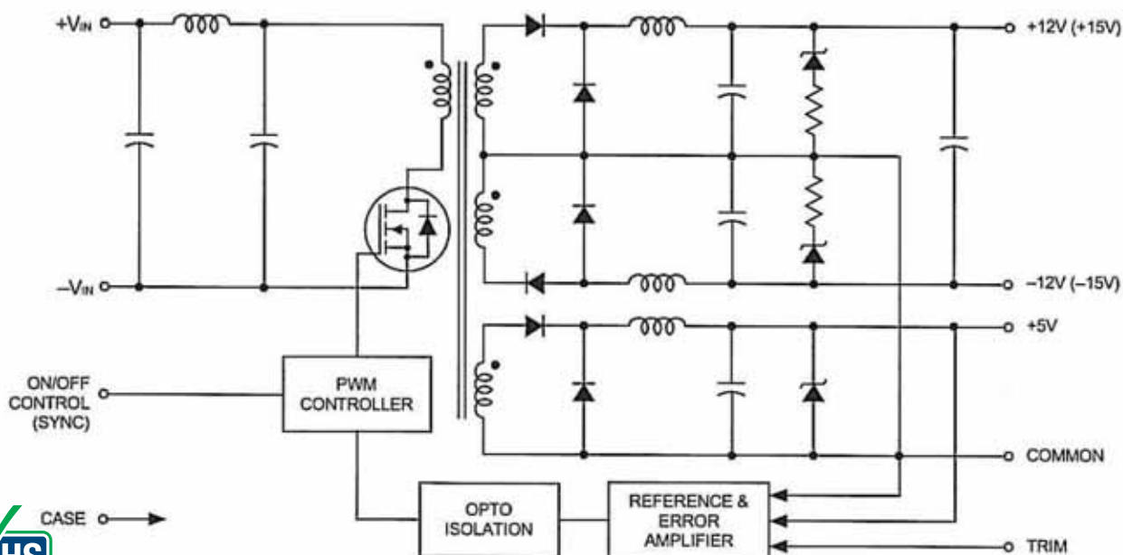
Figure 1. Simplified Schematic
