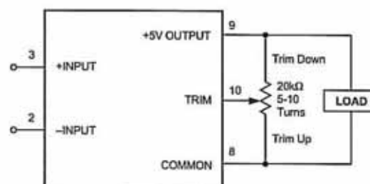
Figure 7. Trim Connections Using a Trimpot
