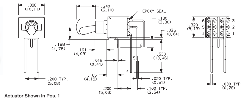
ET21MD1AVBE Vertical Actuation DPDT
