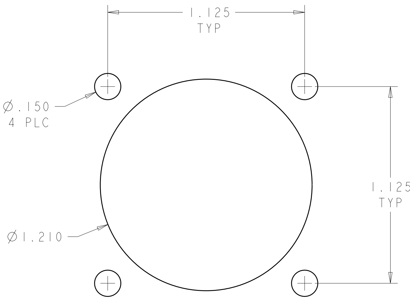
RECOMMENDED PANEL LAYOUT .125 MAX PANEL THICKNESS SCALE 3:1
