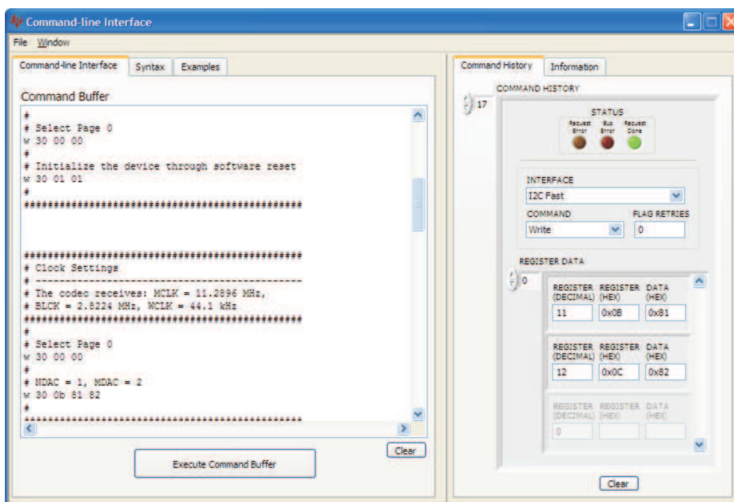
Figure 9. Command Line Interface Panel
