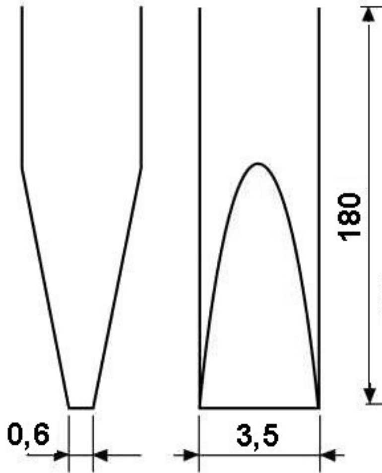
Dimensioned drawing
