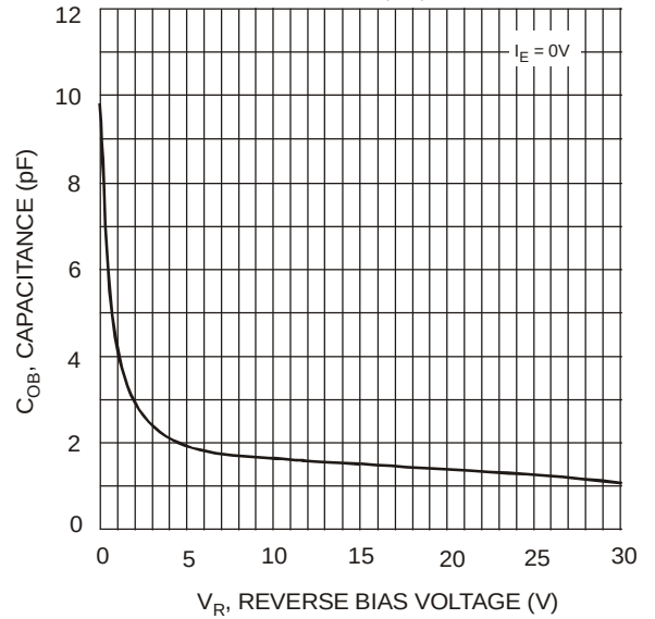
Fig. 4 Output Capacitance
