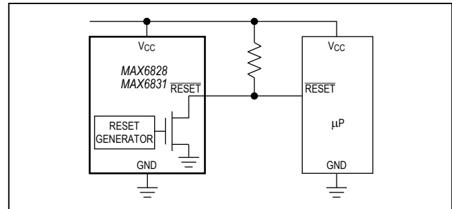
Figure 6. Interfacing Open-Drain \overline{\text{RESET}} to \mu Ps with Bidirectional Reset I/O
