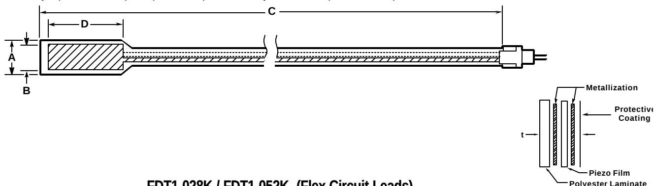
FDT1-028K / FDT1-052K (Flex Circuit Leads)
