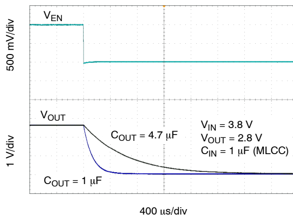
Figure 35. Enable Turn-off
