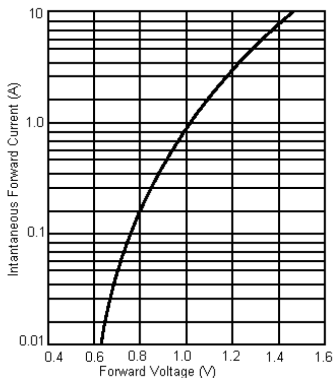
Figure 4 Typical Forward Characteristics
