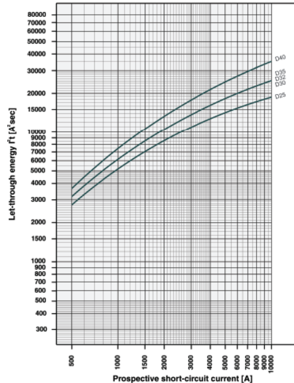
Characteristic D (25 – 40A), 240V
