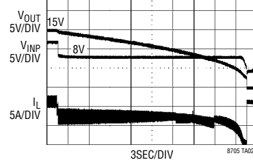
Remove V IN . Loads (4A Draw) Regulated to 8V from Supercaps
