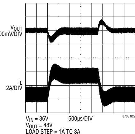
Load Step (Figure 14)
