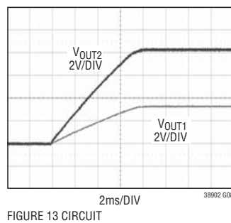
Soft Start-Up
