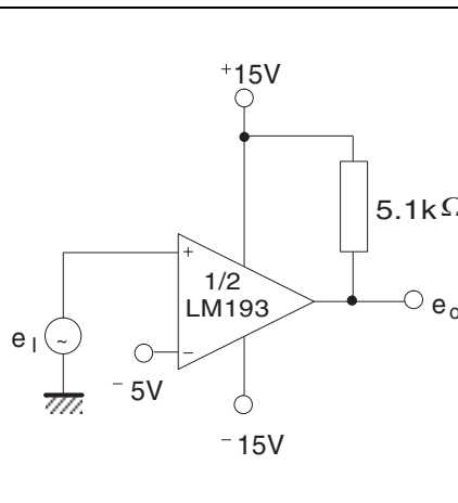
Figure 18. Comparator with a negative reference
