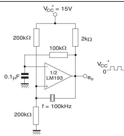
Figure 16. Crystal controlled oscillator
