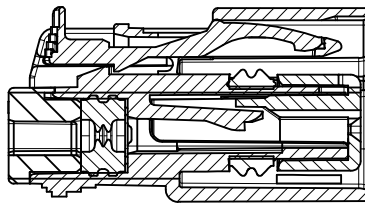
SECTION Y-Y
