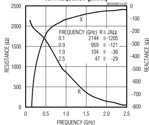
MAX4001 INPUT IMPEDANCE vs. FREQUENCY ( \mu MAX)
