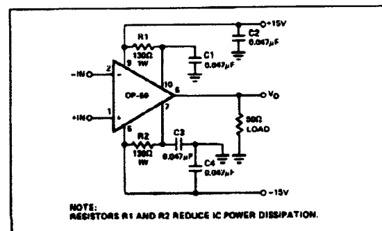
FIGURE 5: DRIVING 50 \Omega LOADS
