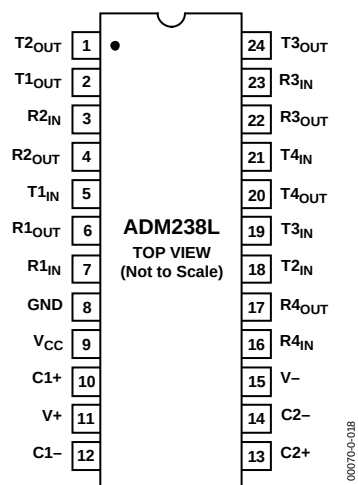
Figure 9. ADM238L PDIP/CERDIP/SOIC Pin Configuration
