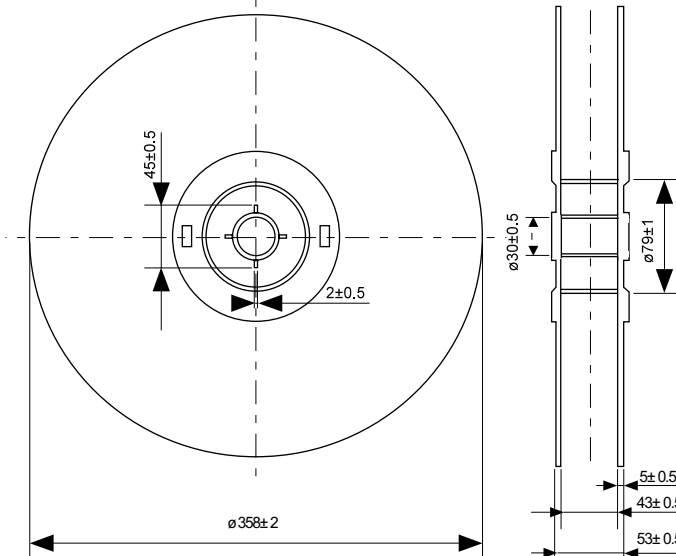
No. YF003-A-R-SD-2.0
