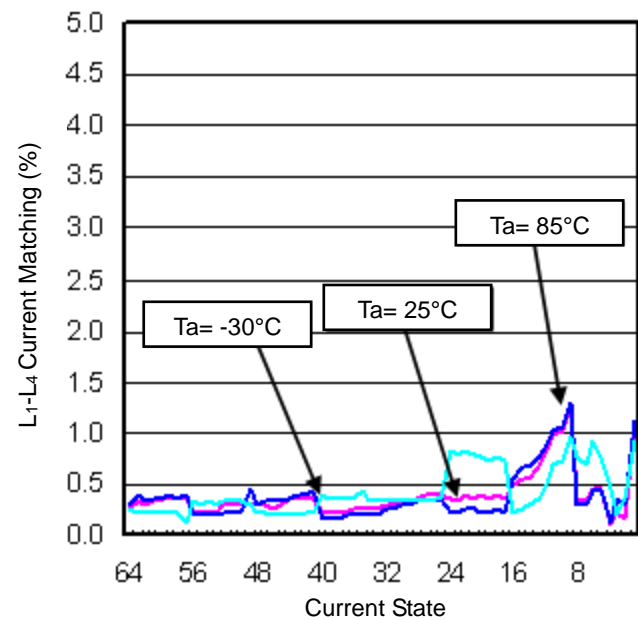
Figure 8. LED Current Relative Accuracy ( V_{IN} = 3.6\text{ V} )
