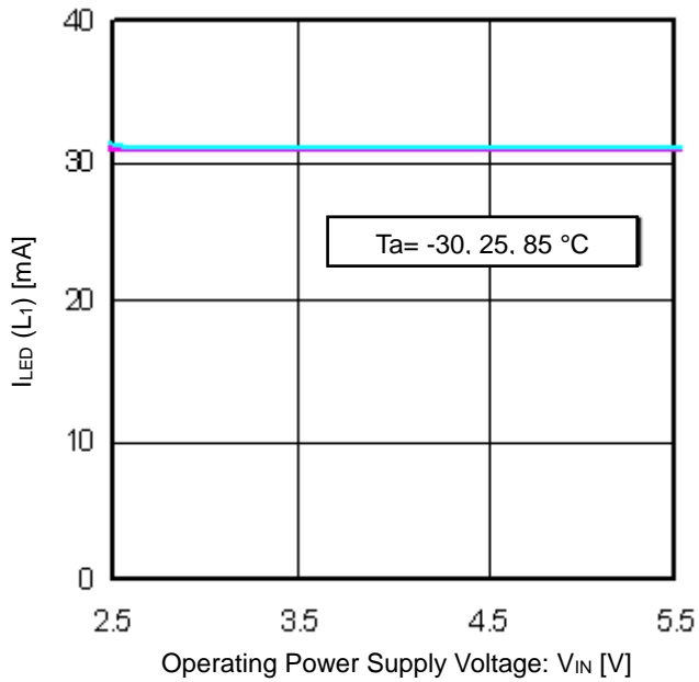
Figure 5. LED Output Current vs Operating Power Supply Voltage ( V_{IN} = 3.6\text{ V} , at 32 mA of LED Current)
