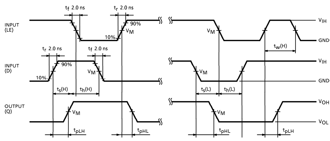
AC WAVEFORM Fig.2 t_{pLH}, t_{pHL}, t_w, t_s, t_h
