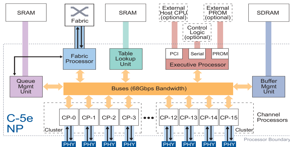
Figure 1 C-5e Network Processor Block Diagram
