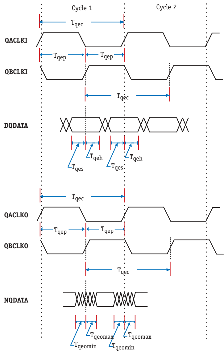
Figure 27 QMU External Mode Timing Diagram
