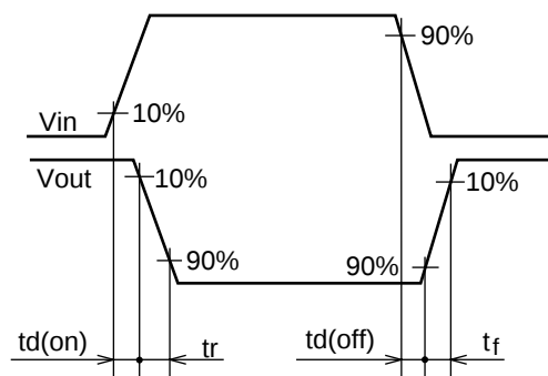
Switching Time Waveforms
