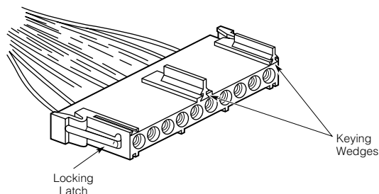
Plug Housing (Accepts Socket Contacts)
