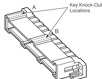
Right-Angle Pin Header
