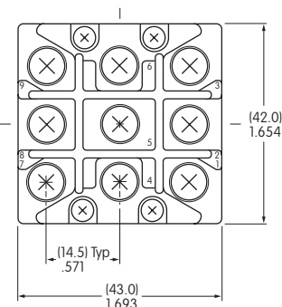
Three Pole
