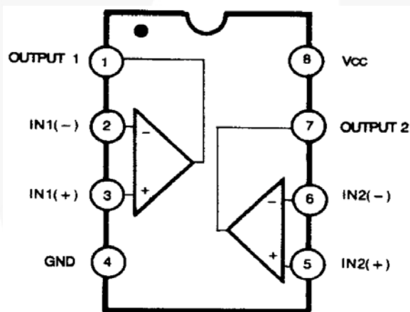
Figure 3. Block Diagram
