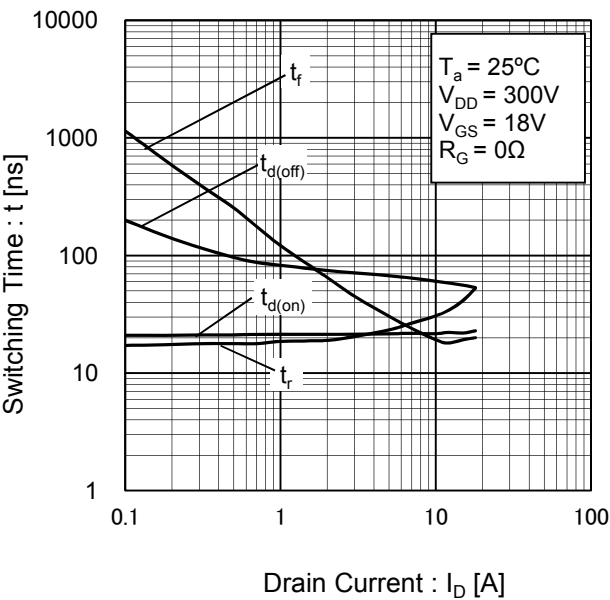
Fig.17 Switching Characteristics
