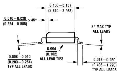
8-Lead (0.150" Wide) Molded Small Outline Package (SOP), JEDEC Order Number LM75AIM, LM75AIMX, LM75CIM-3, LM75CIMX-3, LM75CIM-5, LM75CIMX-5, LM75BIM-3, LM75BIMX-3, LM75BIM-5, or LM75BIMX-5 NS Package Number M08A
