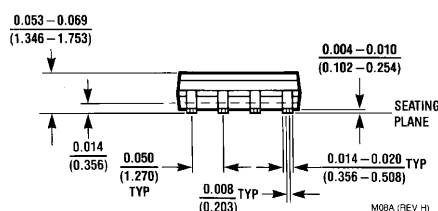
8-Lead (0.150" Wide) Molded Small Outline Package (SOP), JEDEC Order Number LM75AIM, LM75AIMX, LM75CIM-3, LM75CIMX-3, LM75CIM-5, LM75CIMX-5, LM75BIM-3, LM75BIMX-3, LM75BIM-5, or LM75BIMX-5 NS Package Number M08A
