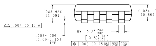
8-Lead Molded Mini Small Outline Package (MSOP) (JEDEC REGISTRATION NUMBER M0-187)
