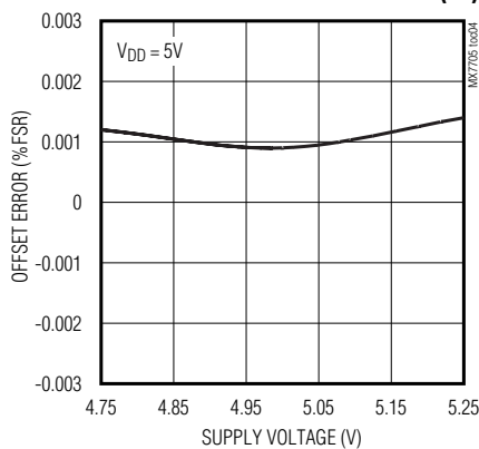
OFFSET ERROR vs. SUPPLY VOLTAGE (5V)
