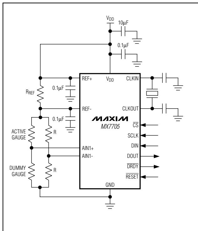
Figure 12. Strain-Gauge Measurement
