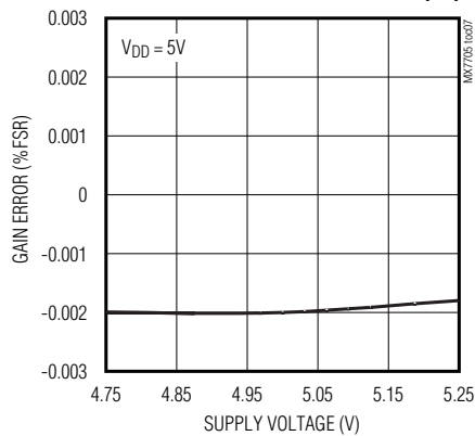
GAIN ERROR vs. SUPPLY VOLTAGE (5V)
