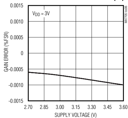
GAIN ERROR vs. SUPPLY VOLTAGE (3V)
