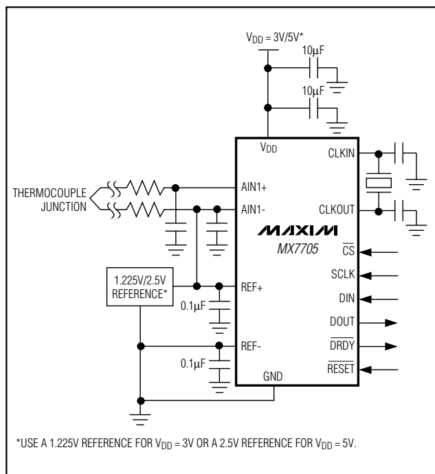
Figure 13. Temperature Measurement
