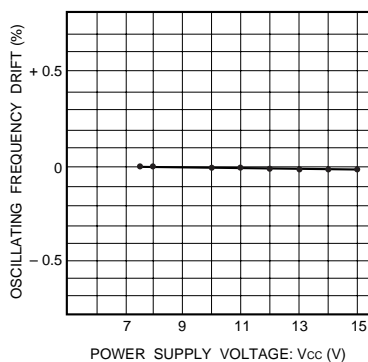
Fig. 4 Oscillation frequency vs. power supply voltage
