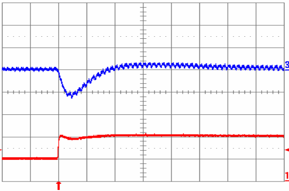
Fig. 1.2V.7: Output voltage response for V_{out} = 1.2 V to positive load current step change from 5 A to 10 A with slew rate of 5 A/ \mu s at V_{in} = 12 V. Top trace: output voltage (100 mV/div.); Bottom trace: load current (5 A/div.). C_o = 100 \mu F ceramic. Time scale: 20 \mu s/div.
