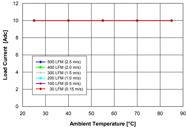
Fig. 1.5V.1: Available load current vs. ambient temperature and airflow rates for V_{out} = 1.5 V converter mounted vertically with V_{in} = 12 V, and maximum MOSFET temperature \leq 110 °C.
