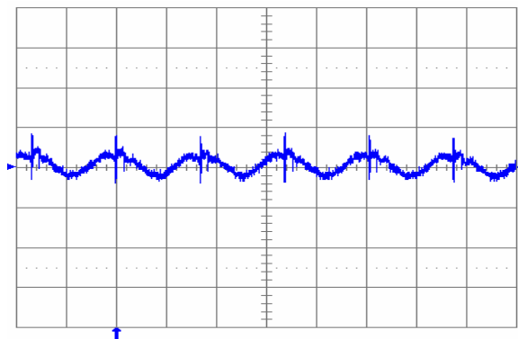
Fig. 0.7525V.6: Output voltage ripple (20 mV/div.) at full rated load current into a resistive load with external capacitance 100 \mu F ceramic + 1 \mu F ceramic, and V_{in} = 12 V for V_{out} = 0.7525 V. Time scale: 2 \mu s/div.
