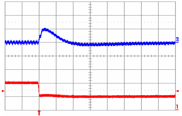
Fig. 1.2V.8: Output voltage response for V_{out} = 1.2 V to negative load current step change from 10 A to 5 A with slew rate of -5 A/ \mu s at V_{in} = 12 V. Top trace: output voltage (100 mV/div.); Bottom trace: load current (5 A/div.). C_o = 100 \mu F ceramic. Time scale: 20 \mu s/div.
