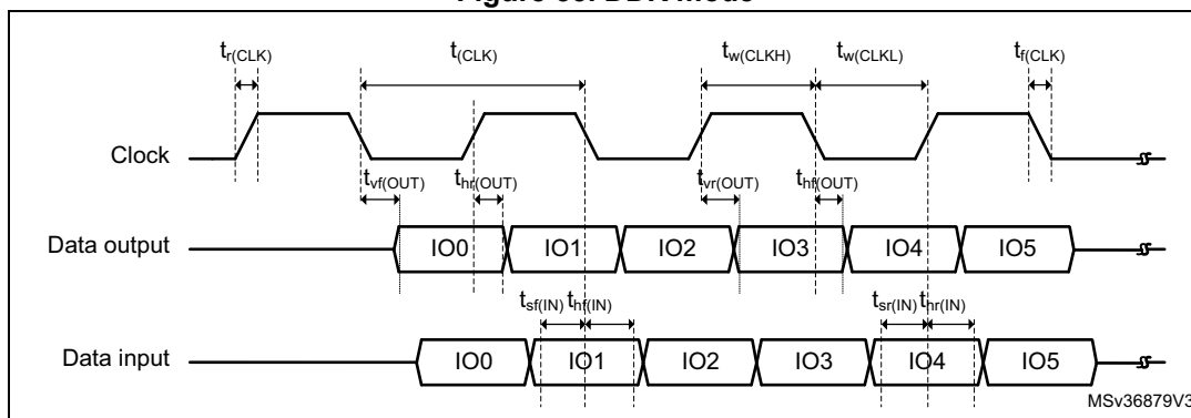
Figure 55. DDR mode
