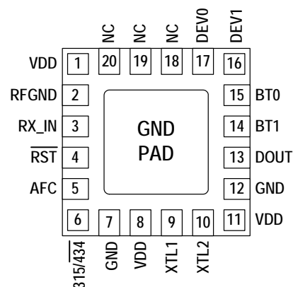
Si4311 (Top View)
