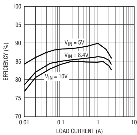
Efficinecy vs Load Current
