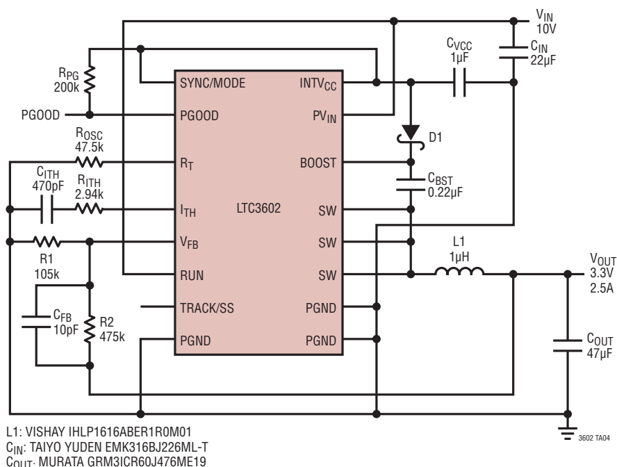
3.3V, 2.5A Regulator at 2MHz, Forced Continuous, Small Size
