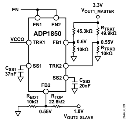
Figure 39. Example of a Ratiometric Tracking Circuit
