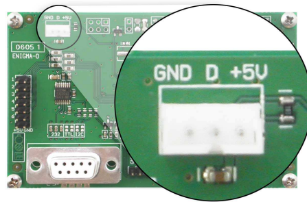
Figure 19: Dallas 1-Wire Bridge
