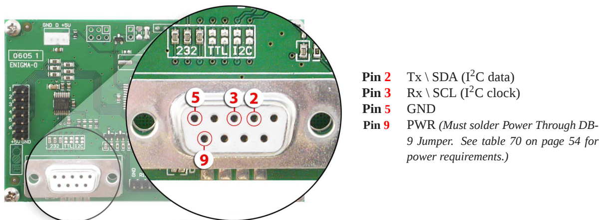
Figure 14: RS-232 Pin out
