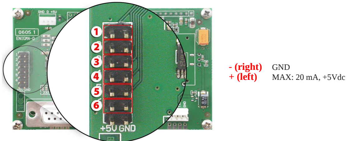
Figure 18: General Purpose Output
