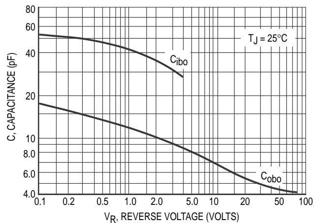
Figure 3. Capacitance
