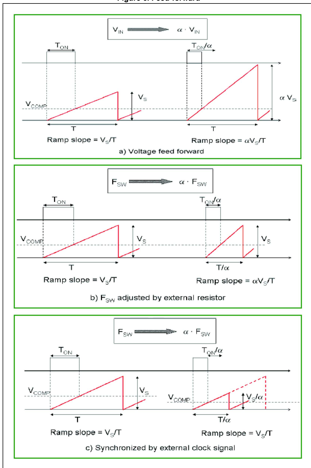
Figure 6. Feed-forward
