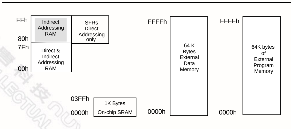
Figure 1. Memory Map
