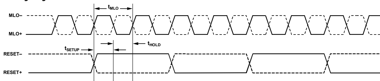
Figure 3. CW Doppler Mode Input MLO_{\pm} , Continuous Synchronous RESET_{\pm} Timing, Sampled on the Falling MLO_{\pm} Edge, 4LO Mode
