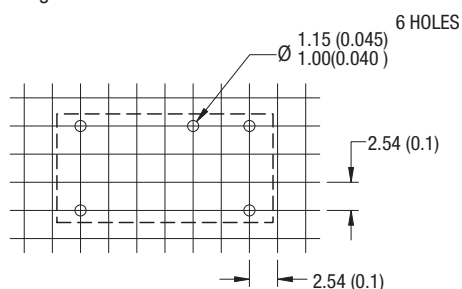
14 Pin DIP Package
