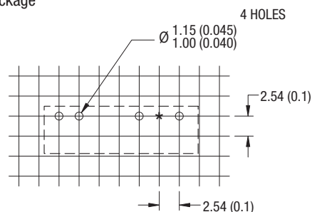
7 Pin SIP Package
