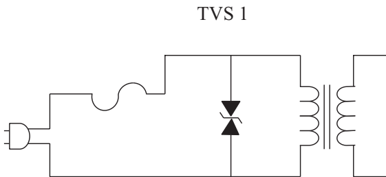
Fig. 5 The bi-directional TVS before bridge rectifier provides an excellent protection to the bridge rectifier.
