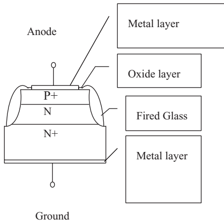
Fig. 2 Cross section of chip for unidirectional TVS
