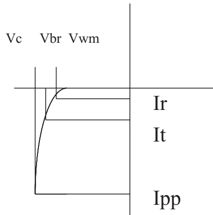
Fig. 3 Unidirectional TVS characteristic curve.
