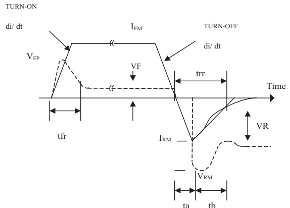
Figure 1. Both typical turn-on and turn-off waveforms of diode.
