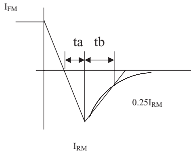
Figure 2-a. Soft- recovery
