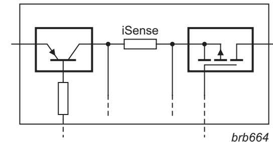
Linear charging
