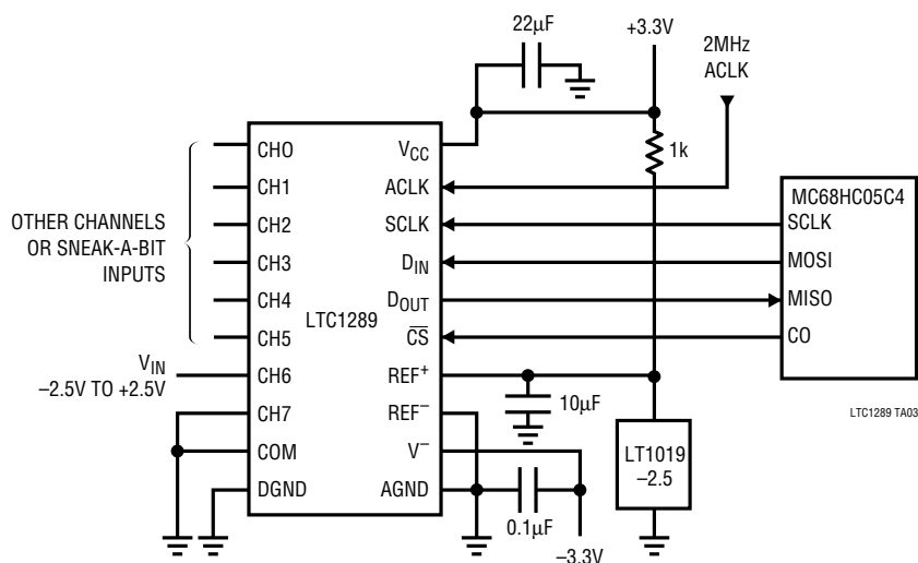
SNEAK-A-BIT Circuit
