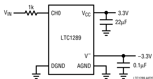
Figure 20. Overvoltage Protection for MUX
