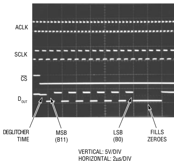
Scope Trace of LTC1289 “Quick Look” Circuit Showing A/D Output of 0101010101 (555 HEX )
