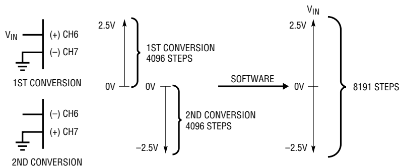
SNEAK-A-BIT
