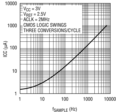
Power Consumption with Power Shutdown vs f_{SAMPLE}
