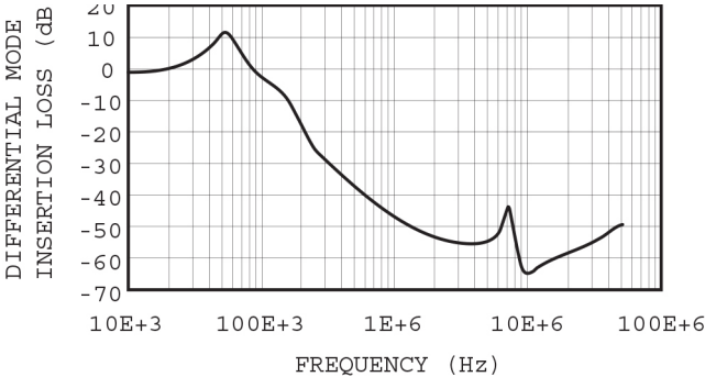
Figure 2. Typical Common-Mode Insertion Loss in a 50 \Omega Circuit
