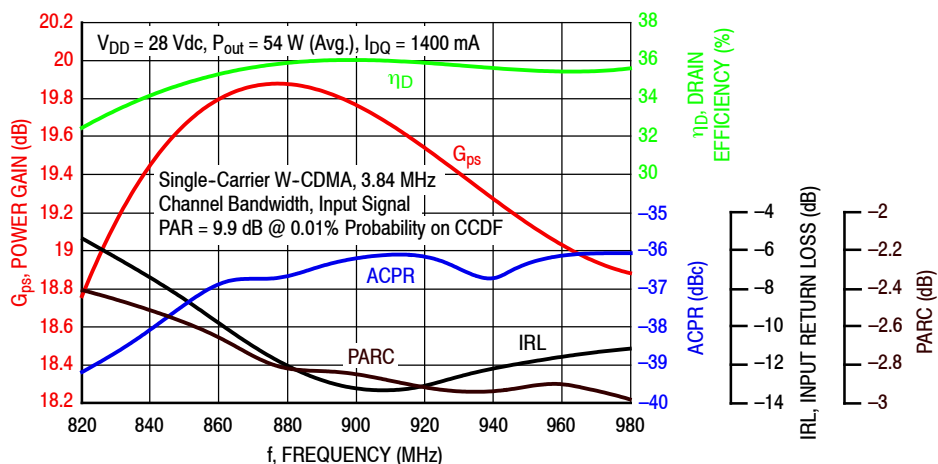
Figure 3. Single-Carrier Output Peak-to-Average Ratio Compression (PARC) Broadband Performance @ P_{out} = 54 \text{ Watts Avg.}
