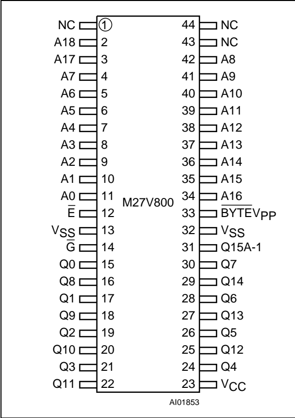
Figure 2C. SO Connections
